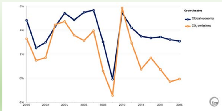
Figure 2 – CO 2 emissions and global economy growth rates
