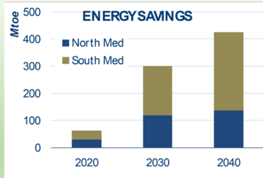
Figure 5 – MEDENER transition scenario compared to conservative scenario
