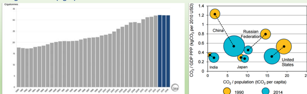
Figure 1 – Global carbon dioxide emissions, 1980-2016 (left), and trends in CO 2 emission intensities for the top five emitting countries* (right)
