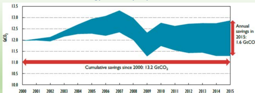
Figure 3 – Avoided GHG emissions from energy efficiency improvements in IEA countries, 2000-2015
